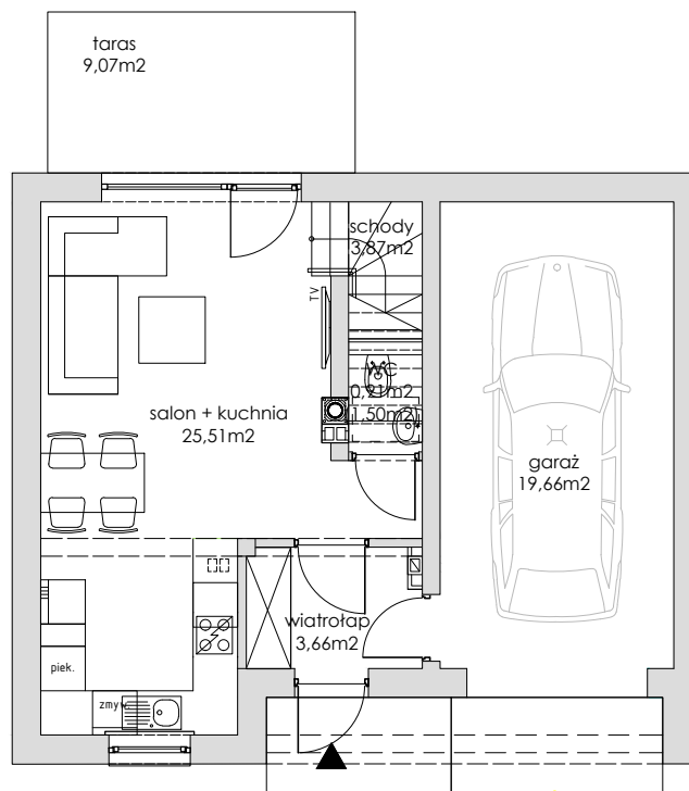
Parter
